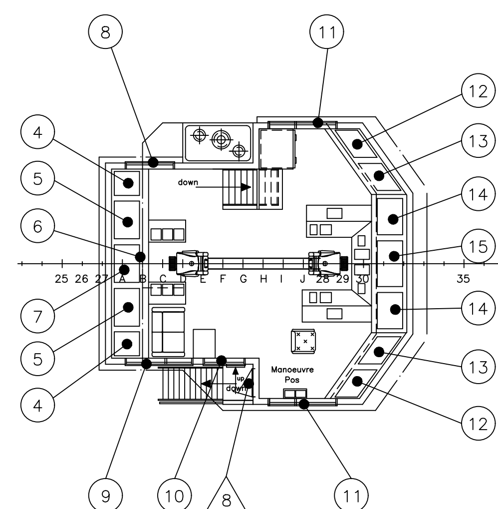
WHEEL HOUSE.
