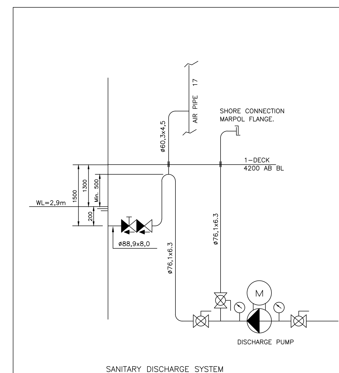
SANITARY DISCHARGE SYSTEM
