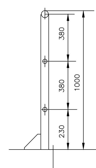
TYPICAL SECTION GUARDRAILS ON DECK.
